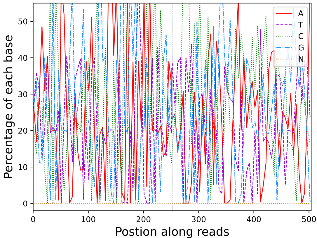
Base percentage along reads (R10911)
